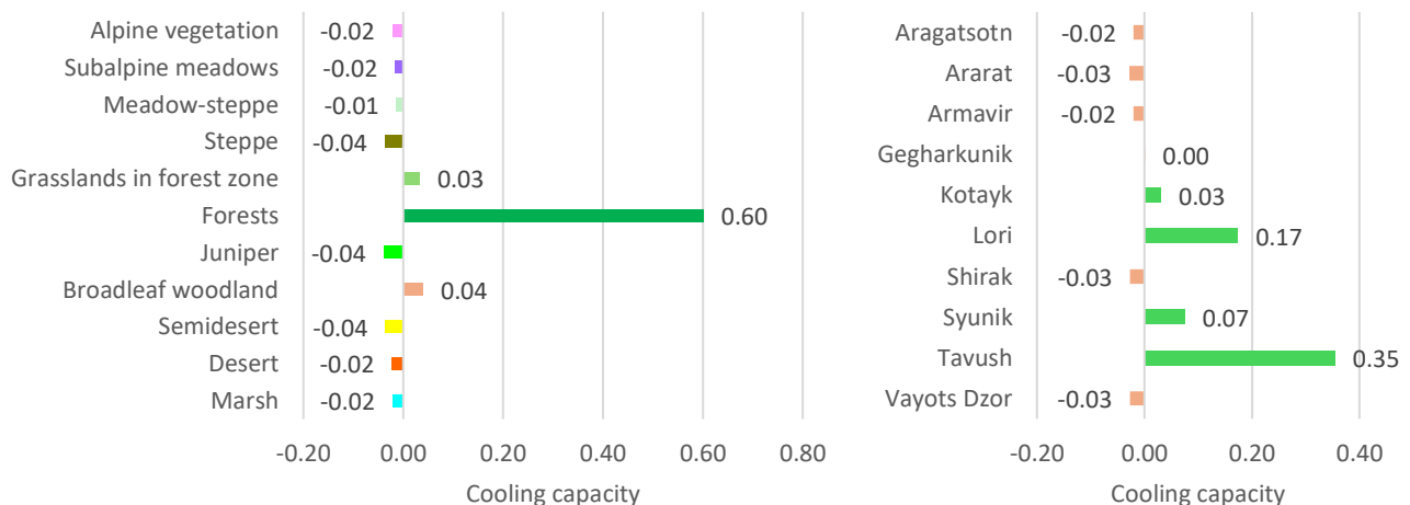
Figure 20. Cooling capacity of different vegetation types (left) and across marzes (right)
