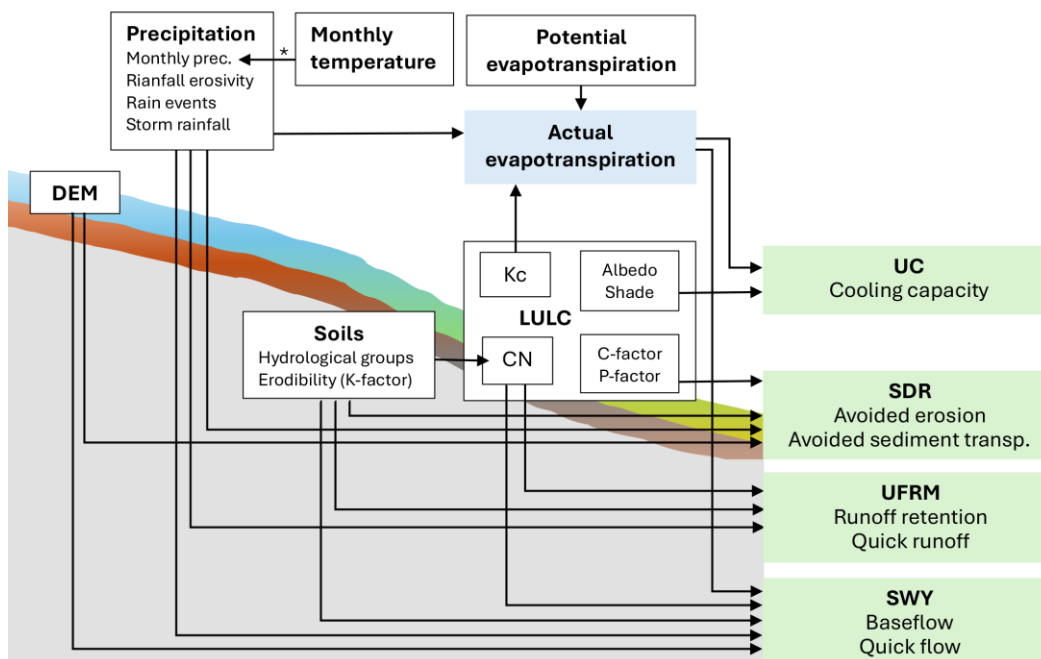
2207 2208 Figure 5.3-1 The relationship between the coefficients used in the tested models. *Average monthly temperature values 2209 were used to adjust the average monthly precipitation, taking into account the snow season.
