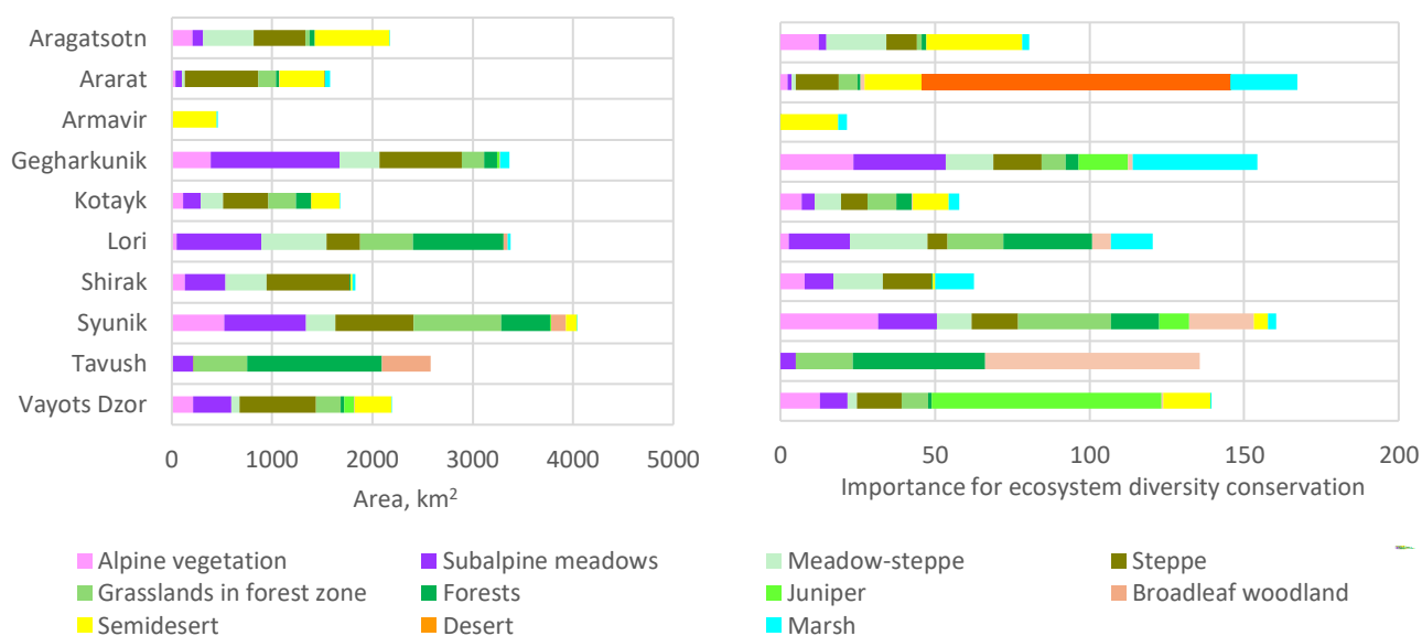
Figure 6. Ecosystem extent across marzes (left) and marz importance for conserving ecosystem diversity in Armenia by the sum of the shares (%%) of the national area of ecosystem types that are conserved within the marzes (right).
