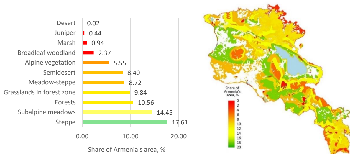
Figure 5. Ranking of ecosystems by rarity (left) and rarity map of ecosystems (right). White color indicates anthropogenic areas
