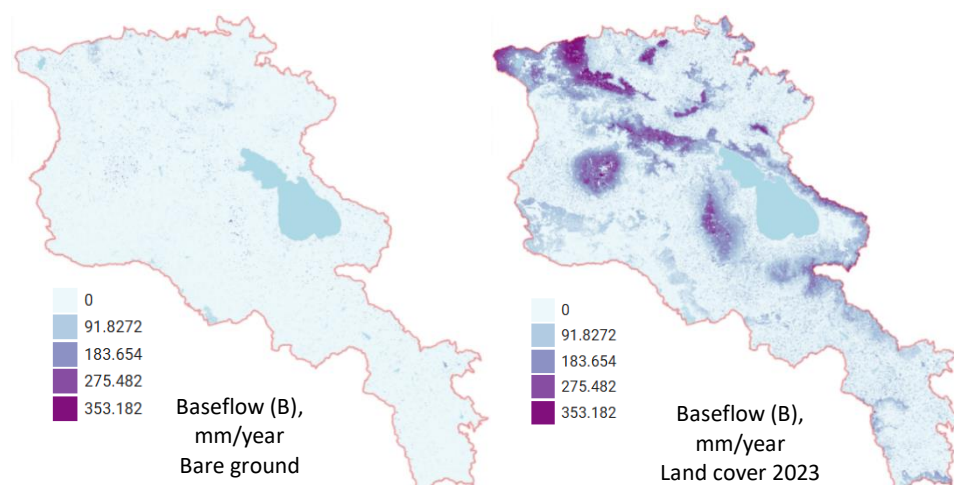
Figure 2. Baseflow on bare ground and under current land cover
