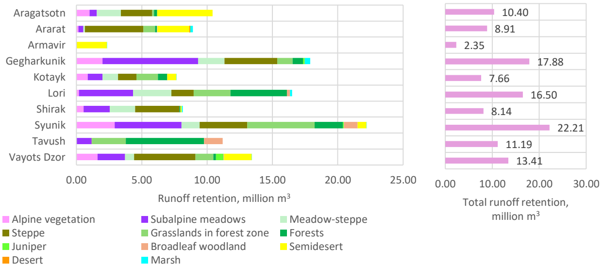
Figure 23. Runoff retention provided by ecosystems across marzes
