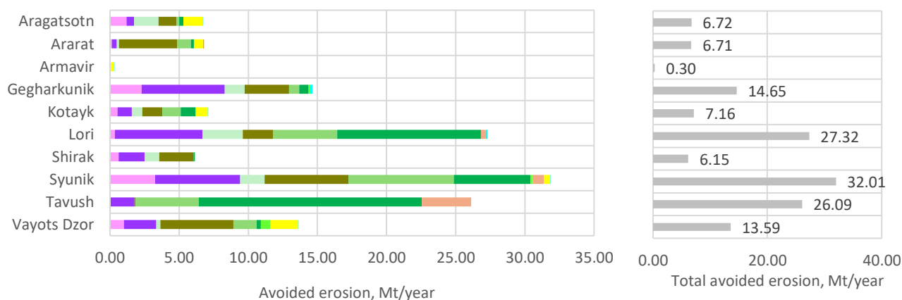
Figure 26. Avoided erosion across marzes
