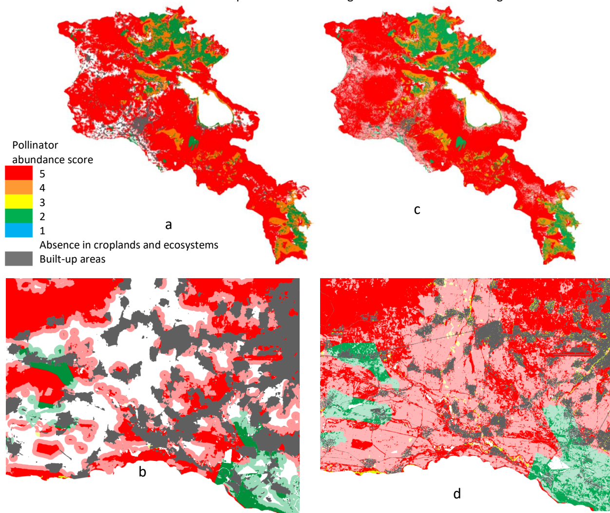
Figure 3.1.H-6. Pollination zones of Hymenoptera : (a, b) based on the Esri 2023 data; (c, d) based on the ESA 2021 data. The 460 m buffer within agricultural fields, representing areas reached by Hymenoptera from natural ecosystems, is shown in lighter colours. Enlarged map fragments of part of the Ararat Valley are presented at the bottom.
