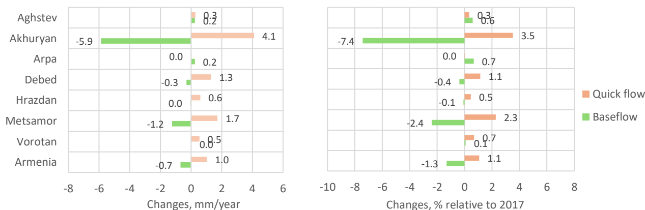
Figure 3.1.B3-2. Changes in baseflow and quickflow from 2017 to 2023 in absolute (a) and relative (b) indicators across watersheds
