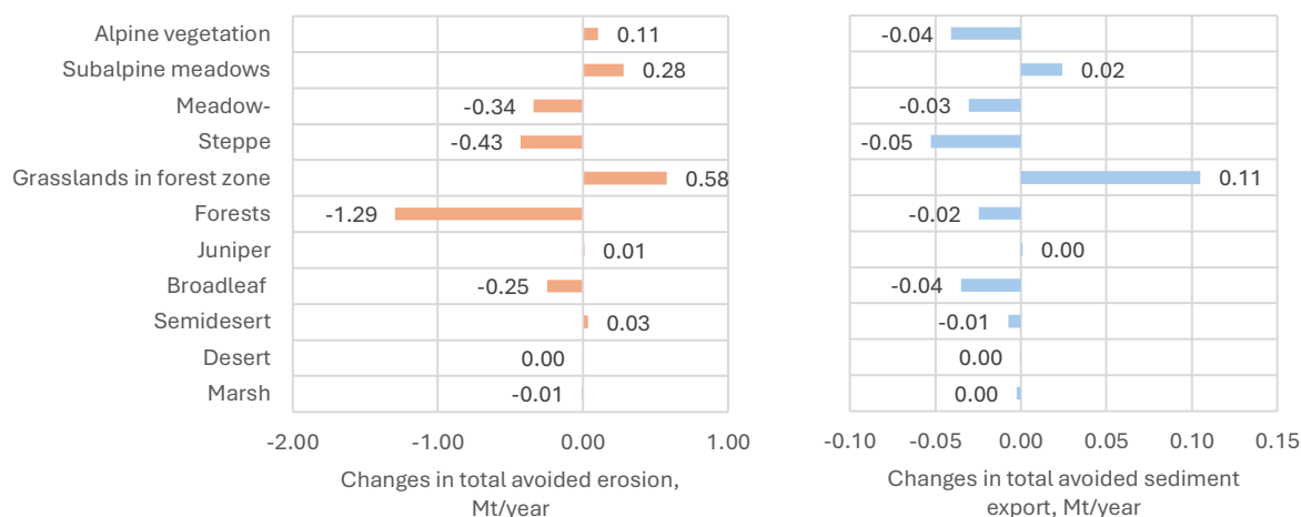
Figure 3.1.C2-3. Changes in avoided erosion and avoided sediment export across vegetation types in the whole Armenia.
