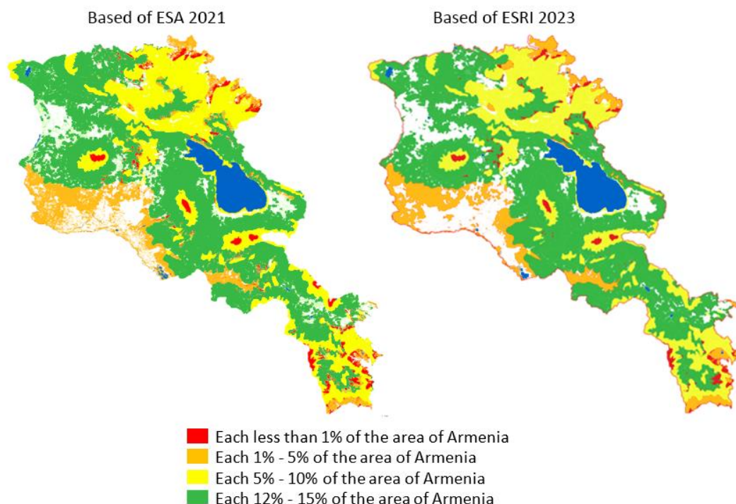
Figure 2.5.A-3. Maps of LLCC rarity based on ESA and Esri land cover datasets
