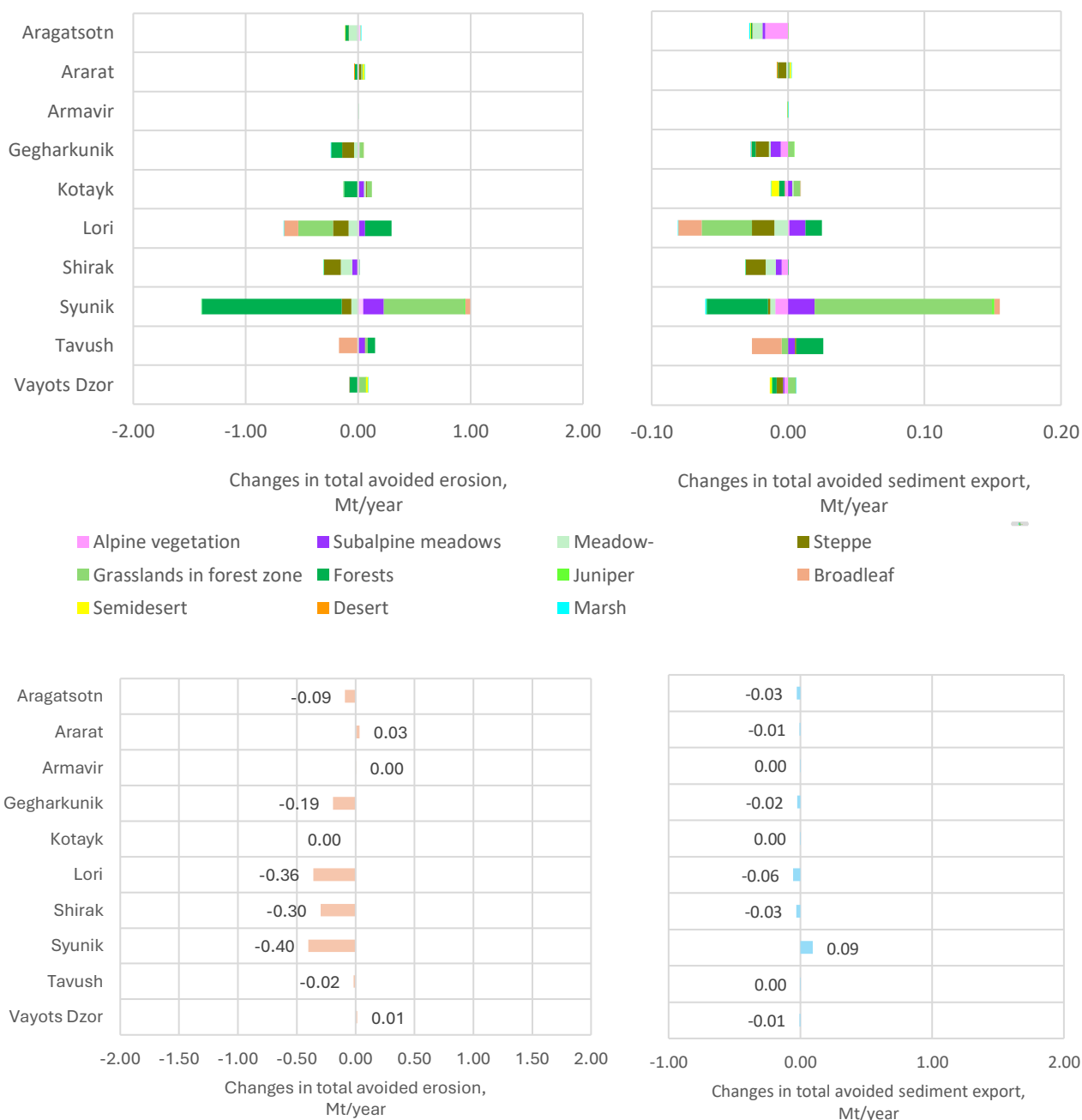
Figure 3.1.C2-2. Changes in avoided erosion and avoided sediment export across vegetation types and marzes.
