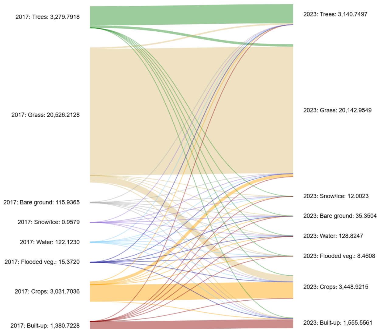
Figure 2.2.B-6. Transitions between land cover classes from 2017 to 2023
