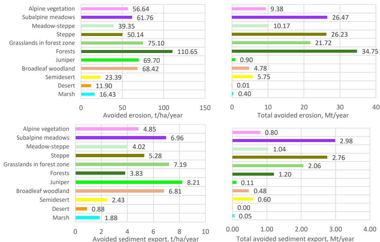
Figure 3.1.C1-4. ES indicators across vegetation types
