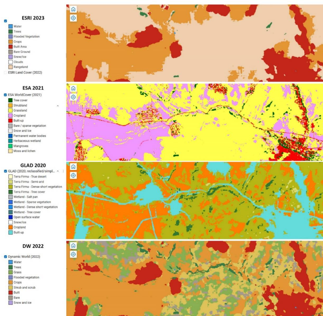
Figure 2.1.A-6. The same area as represented in different land cover datasets
