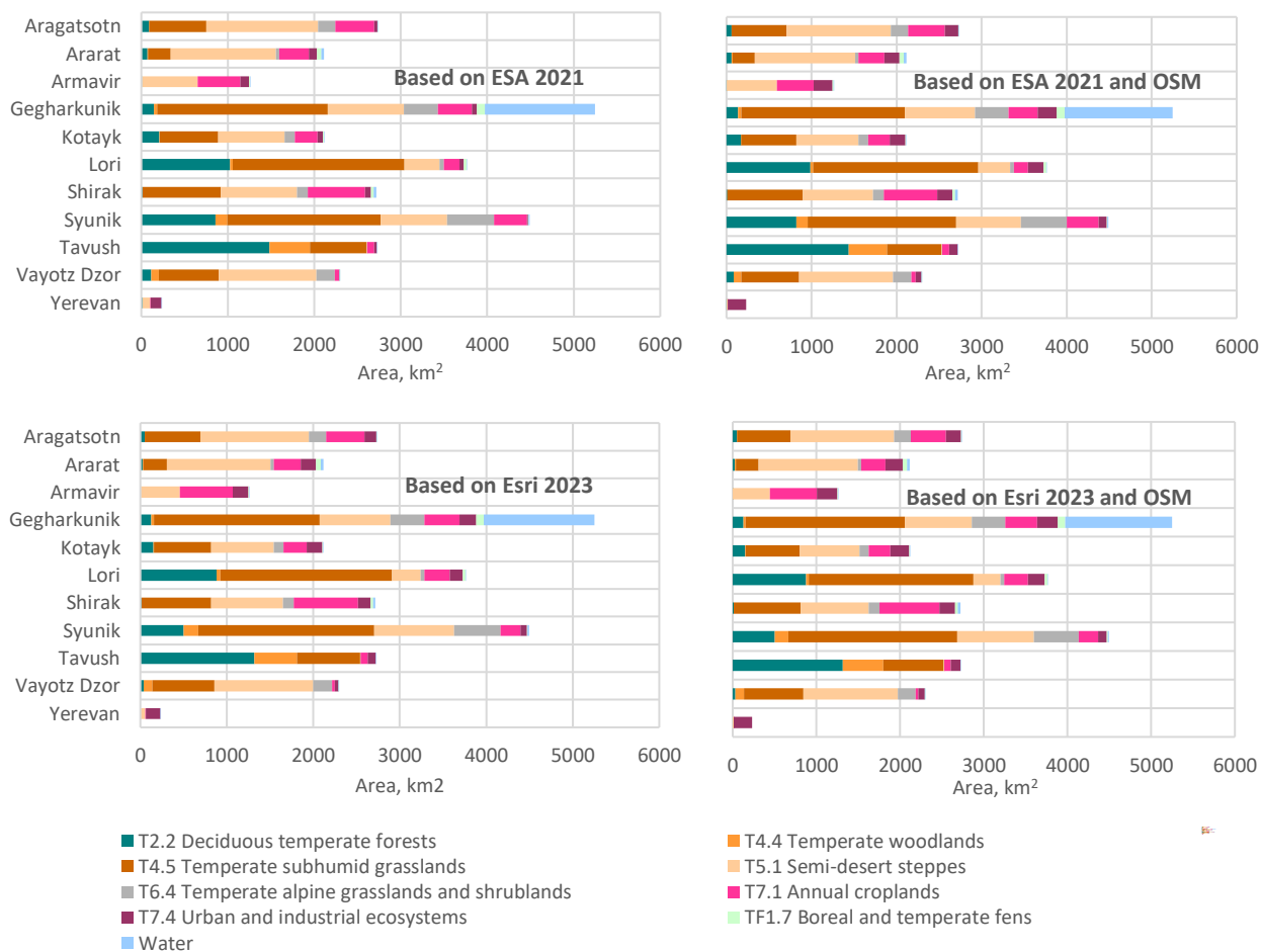
Figure 2.7.B. Ecosystem area in Armenia and across marzes in different versions of ecosystem map, km 2
