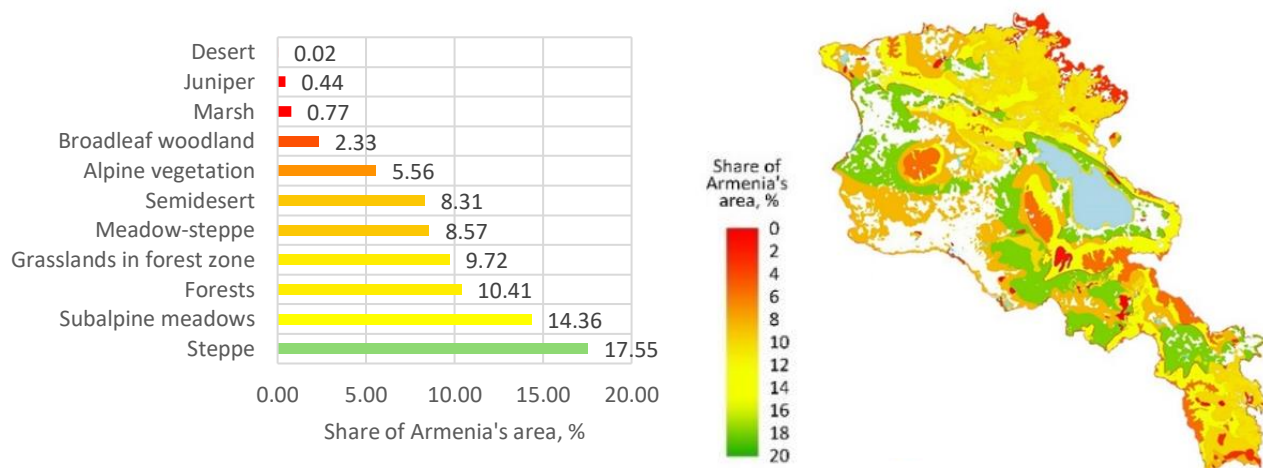
Figure 2.3.B-1. Ranking of ecosystem types by rarity and the map of ecosystem rarity
