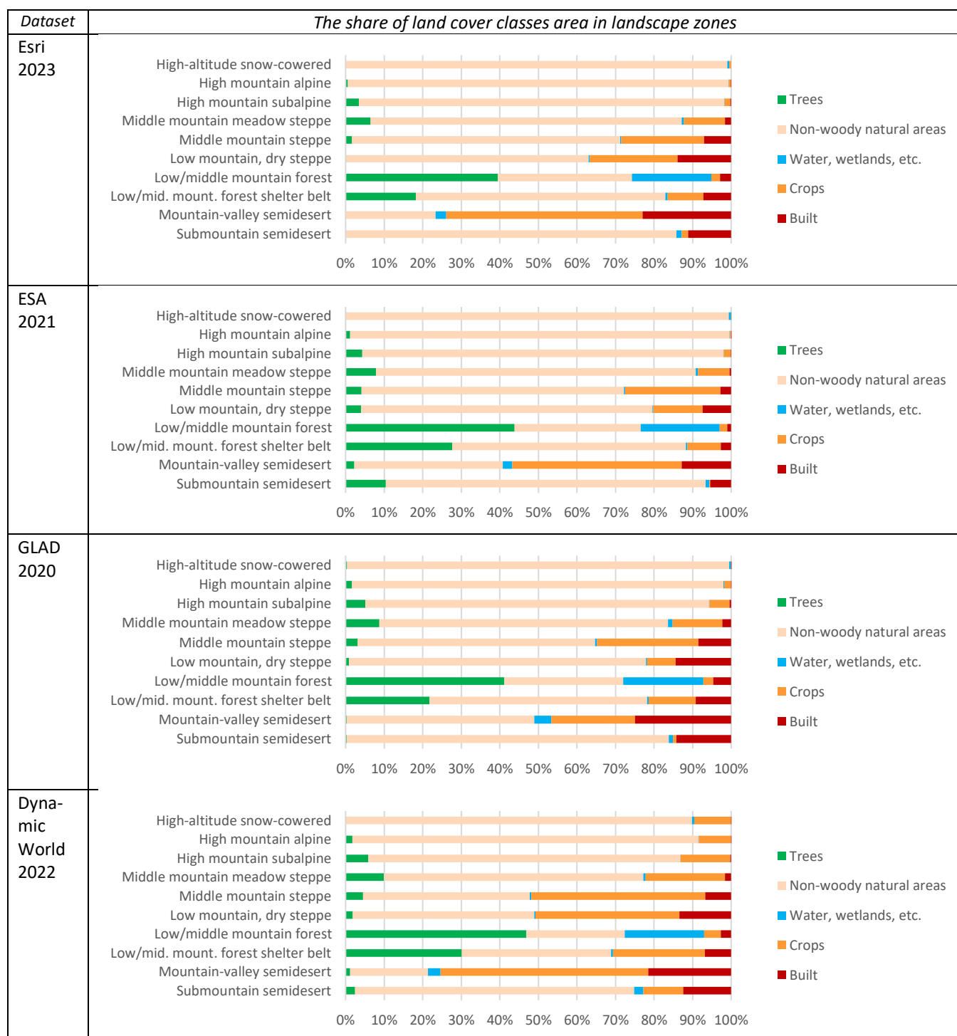
Figure 2.1.A-9. Land cover class shares across landscape zones according to tested datasets
