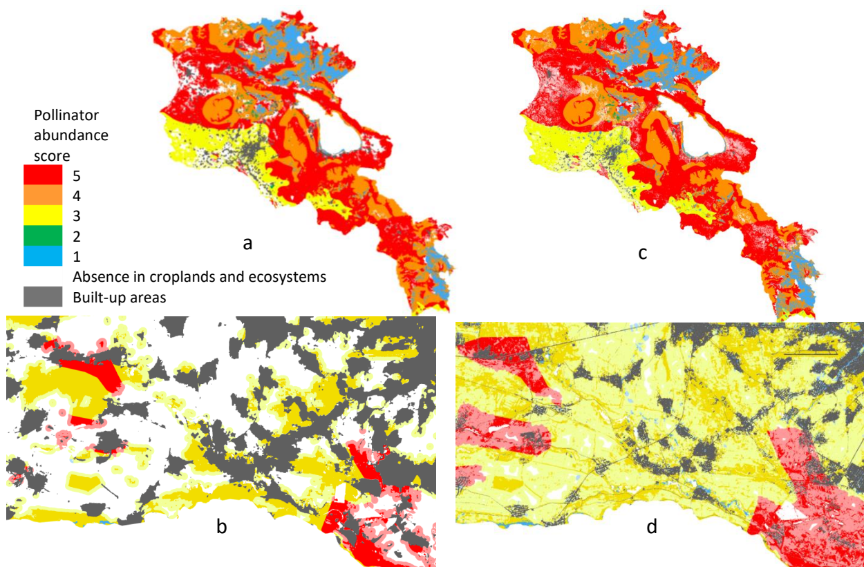
Figure 3.1.H-8. Pollination zones of Diptera : (a, b) based on the Esri 2023 data; (c, d) based on the ESA 2021 data. The 460 m buffer within agricultural fields, representing areas reached by Hymenoptera from natural ecosystems, is shown in lighter colours. Enlarged map fragments of part of the Ararat Valley are presented at the bottom.
