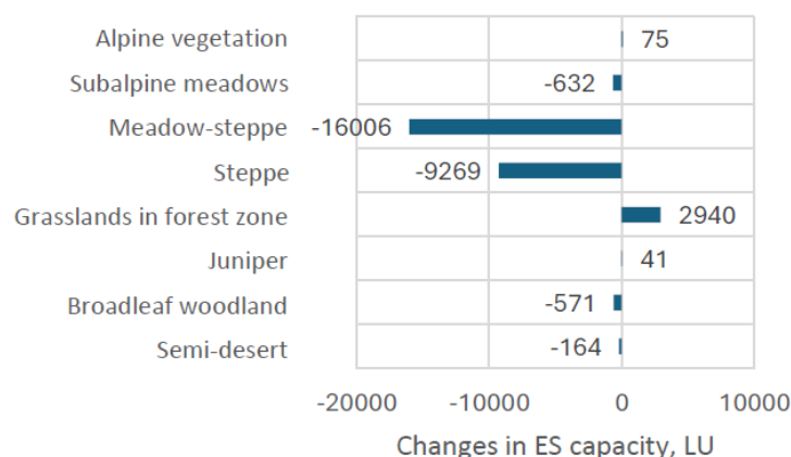
Figure 3.2.A2-1. Changes in ES capacity from 2017 to 2023 in different ecosystem types across marzes
