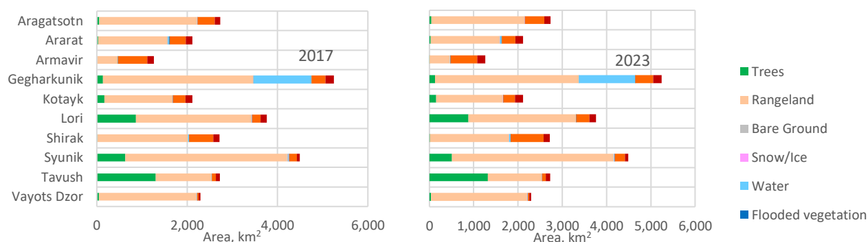
Figure 2.2.B-2. Area of land cover classes in 2017 and 2023, km 2
