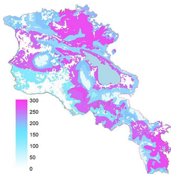
Figure 3.2.B4-8. The map of ES summed score
