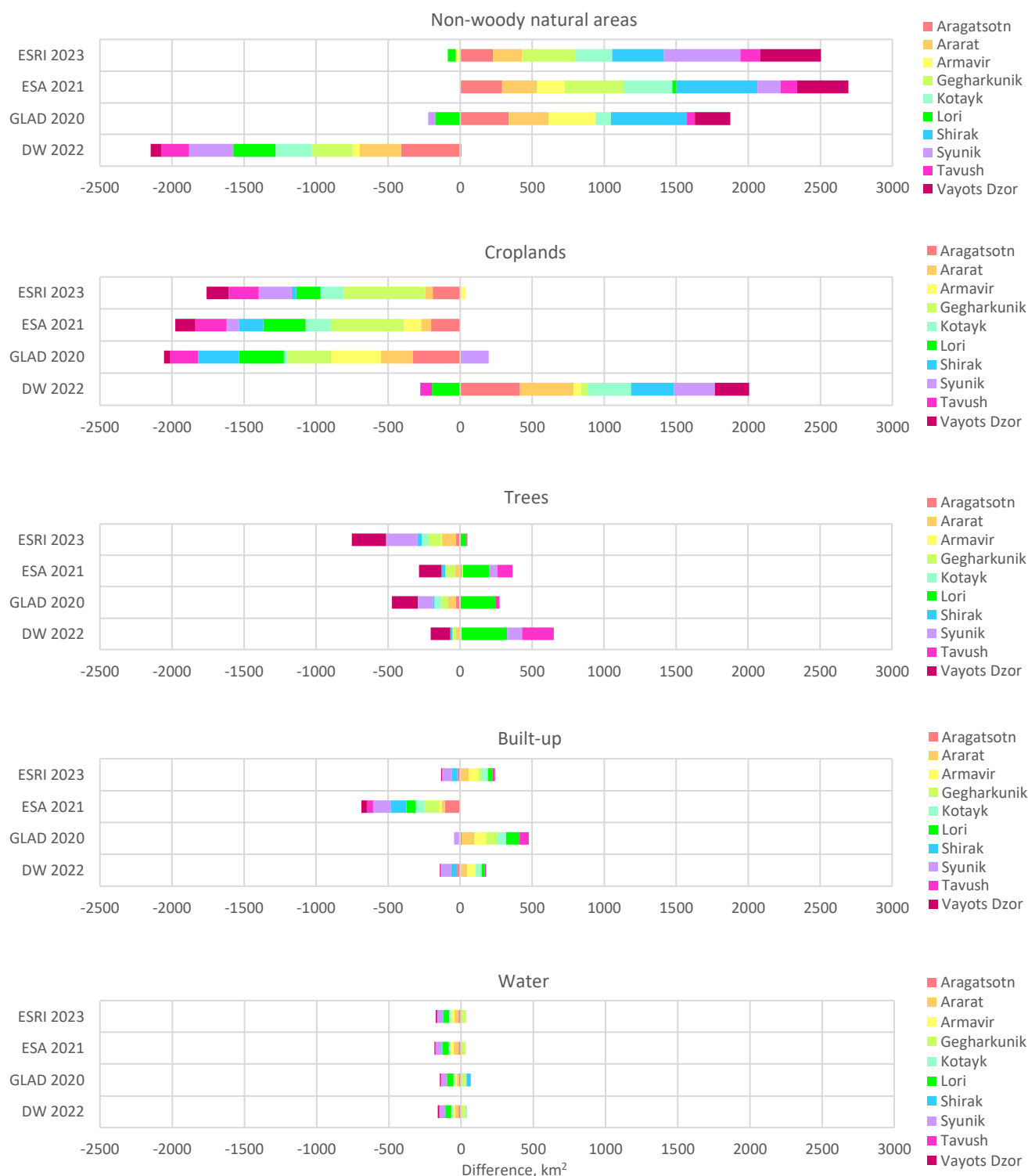
Figure 2.1.A-4. Land cover area difference: Government-reported areas minus areas from tested datasets. Differences between tested datasets and Government-reported data in marzes are shown in different colors. Provincial differences for each land cover class are combined into a single bar to show the total deviation from the Government-reported data.
