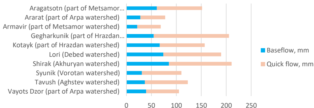
Figure 3.1.B1-4. Baseflow and quick flow under the current land cover across marzes, mm/year
