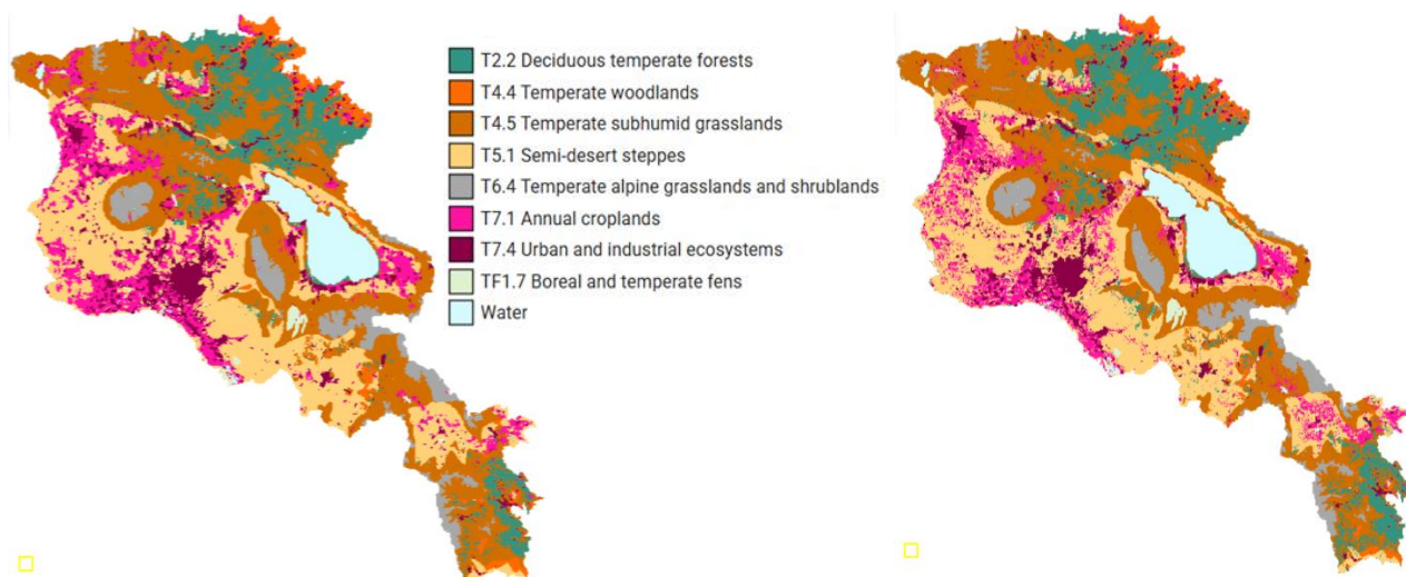
Figure 2.7.A-5. Maps of current terrestrial ecosystems of Armenia based on Esri 2023 and ESA 2021 land cover data and built-up areas from OSM. See details in project WEB GIS
