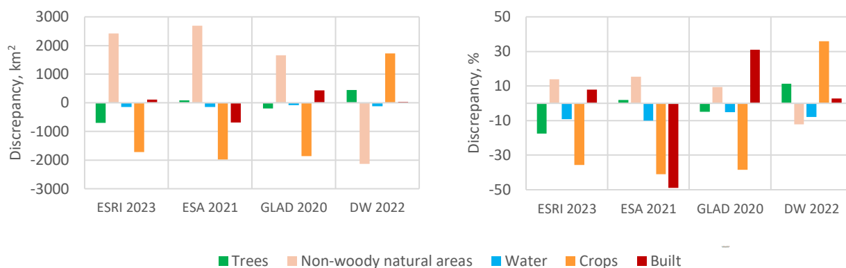
Figure 2.1.A-5. Absolute (km²) and relative discrepancy (% relative to Government-reported data) in area of land cover classes
