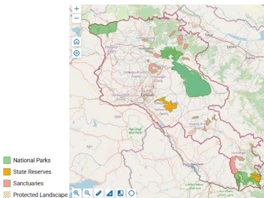
Figure 31I-1. The map of protected areas of Armenia. For details see project Web GIS https://bccarmenia.nextgis.com/ , section "Protected areas" (the location of the Goravan Sands Sanctuary needs to be clarified)
