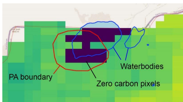
Figure 3.1.I-6. An example of a significant error in estimating carbon content in a small PA is observed in the case of the sanctuary Sev Lich.
