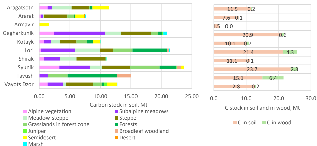
Figure 3.1.G1-2. Carbon stock, MtC in soil in different vegetation types across marzes (a) total C stock in soil and wood across marzes (b). Area of the marz Gegharkunik is accounted excluding Lake Sevan
