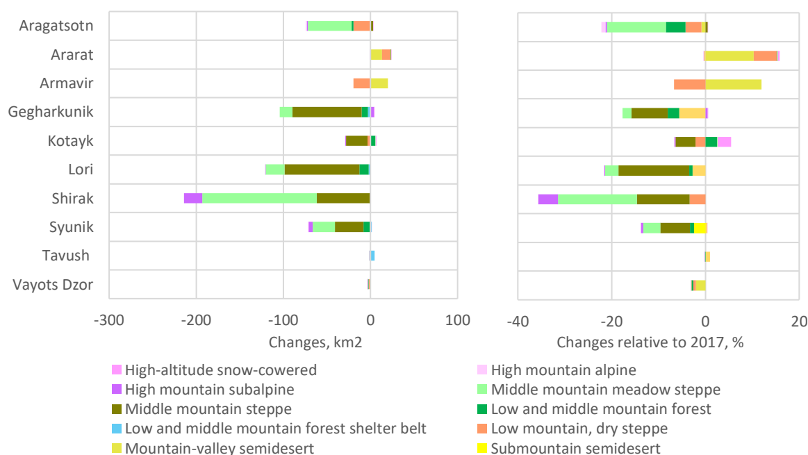
Figure 2.4.C-2. Changes in natural landscape extent from 2017 to 2023, based on Esri data: a) absolute changes, km 2 ; b) share of changed area relative to 2017, %
