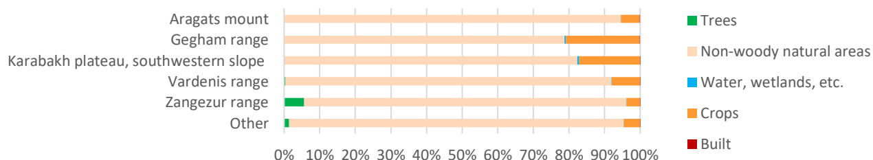
Figure 2.1.A-10. Land cover class shares in high-altitude snow-covered and high mountain alpine zones across highland systems of Armenia according to DW 2022 data
