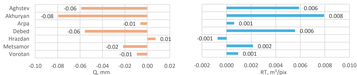
Figure 3.1.D1-2. Ecosystem effect on quick runoff and runoff retention across watersheds under the average spring rainfall scenario (12 mm).
