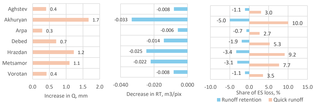
Figure 3.1.D2-3. ES loss resulting from the historical conversion of natural grasslands by humans
