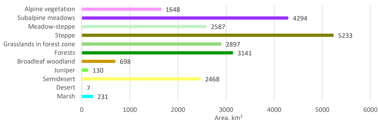
Figure 2.3.A-3. Area of natural ecosystem types, km 2
