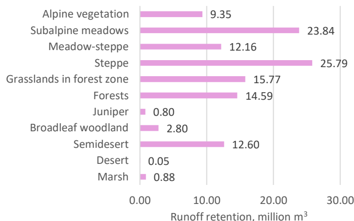
Figure 3.1.D1-8. Total runoff retention provided by different vegetation types, million m³
