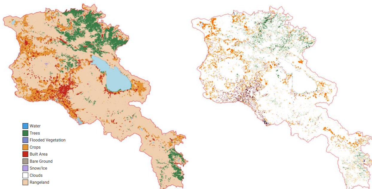
Figure 2.2.B-5. The land cover and its changes: a) Esri land cover data for 2023; b) The land-cover changes that occurred since 2017, specifically the new land-cover classes that emerged in place of previous ones, are shown.
